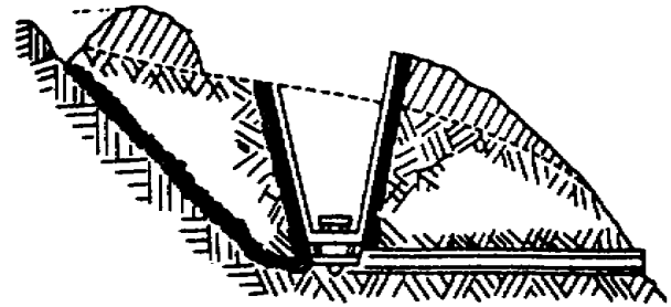
Figure 2-8. Use of undertrench drains.
